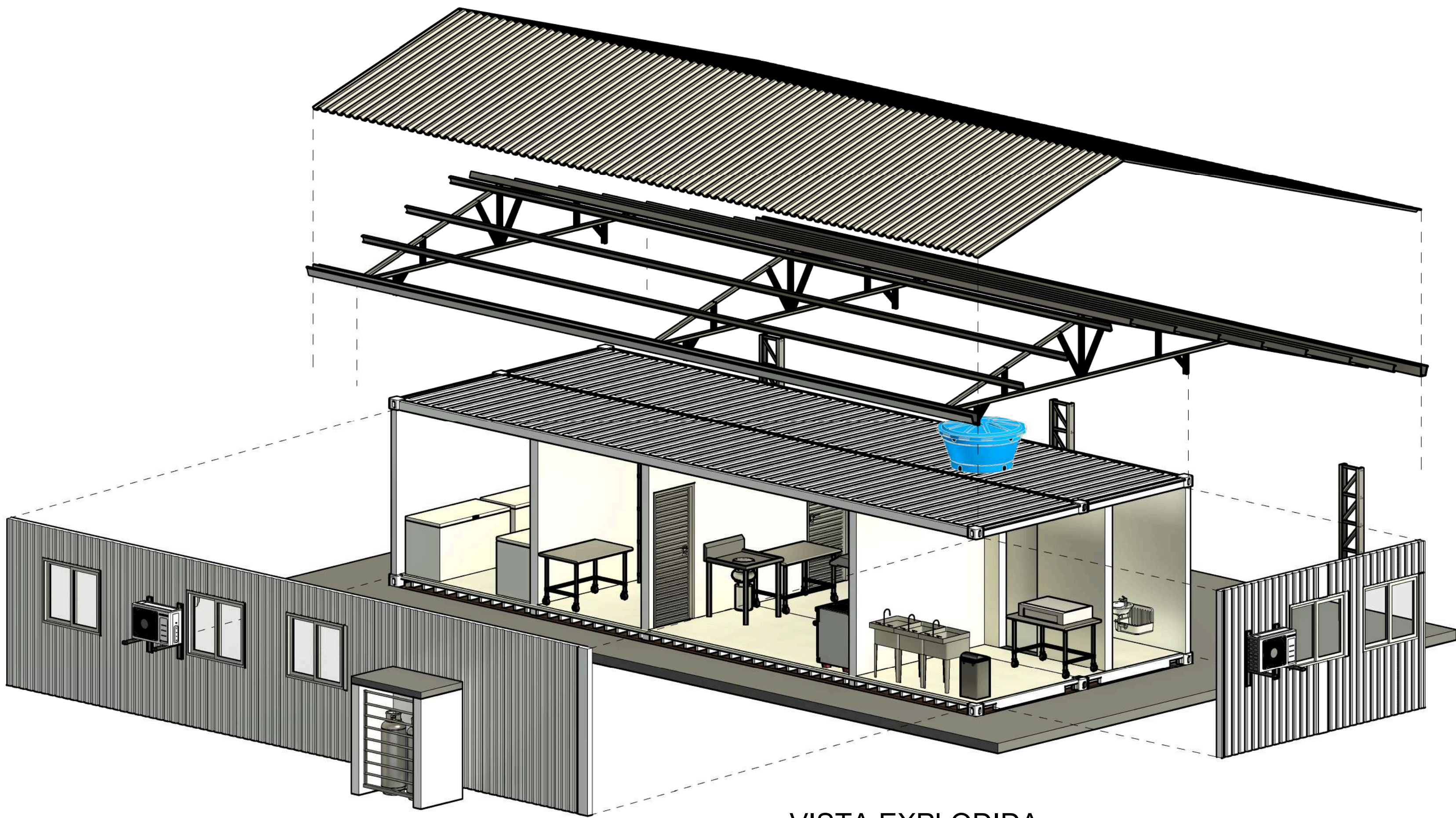
VISTA EXPLODIDA
